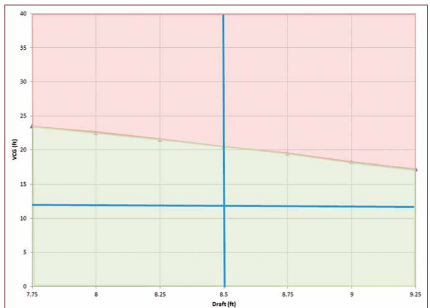
Limiting vertical center of gravity curve example for Hull 1. Coast Guard graphic by Ensign Erin Morgan
