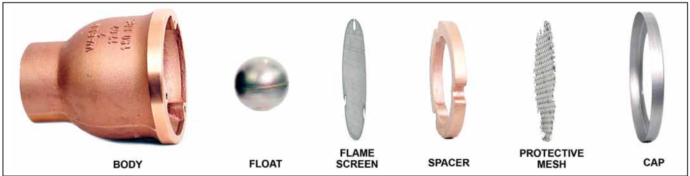
An inverted vent check valve protects tanks and bulkheads from pressure build-up during loading and unloading of liquid or dry cargo and assures maximum efficiency during operations. The ball float prevents contamination of the tank cargo from sea water during heavy seas. Illustration courtesy of Wager Company USA
